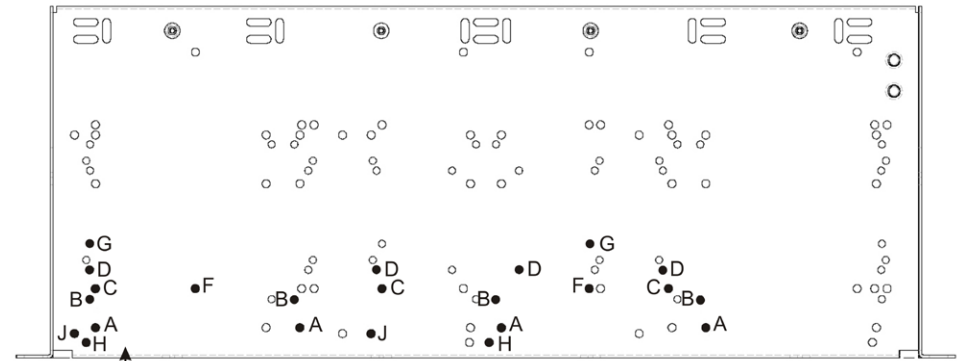
First module/chassis mounting holes
